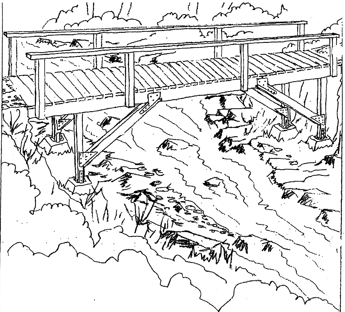
TYPICAL WALKING BRIDGE SCALE: NO SCALE
