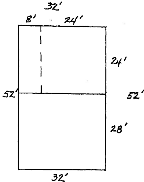
BUILDING FOOTPRINT DIMENSIONS - LOT # 2 SCALE: 1" = 20' ±
