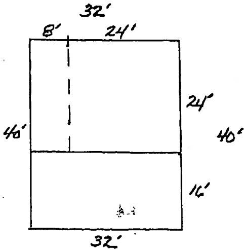
BUILDING FOOTPRINT DIMENSIONAL - LOT # 1 SCALE: 1" = 20' ±
