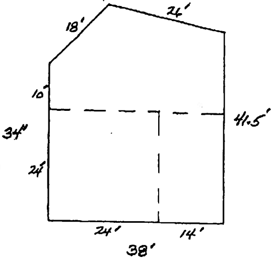
BUILDING FOOTPRINT DIMENSIONAL - LOT # 4 SCALE: 1" = 20'
