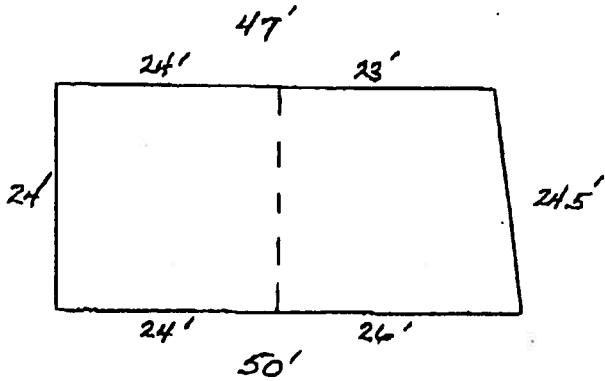
BUILDING FOOTPRINT DIMENSIONAL - LOT #5 SCALE: 1" = 20' ±
